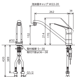
KM5011TEC
