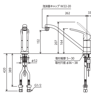
KM5011T
