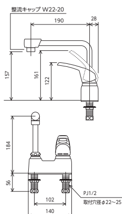
KM7024K
